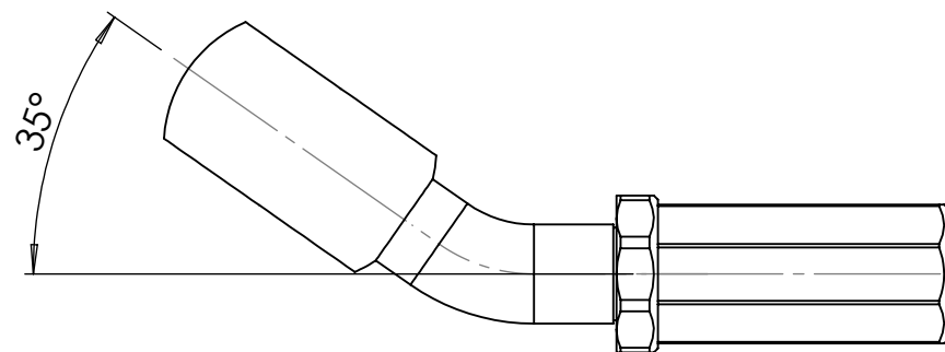
10mm Banjo 35 degrees B10.35.00
