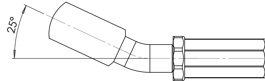
10mm banjo 25 degrees B10.25.00
