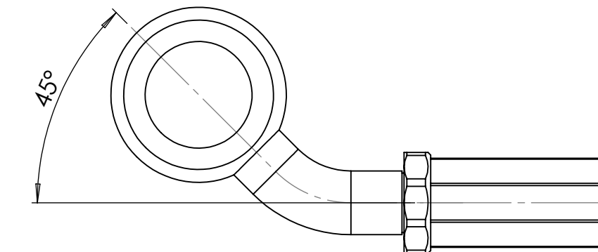
10mm banjo side bend 45 degrees B10.00.45
