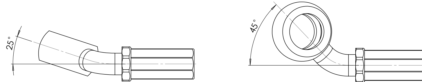
10mm banjo 25 degrees + side bend 45 degrees B10.25.45
