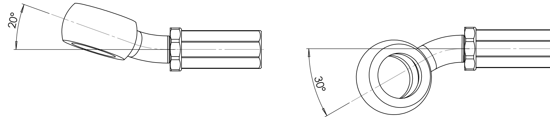
10mm banjo 20 degrees + side bend 30 degrees B10.20.30
