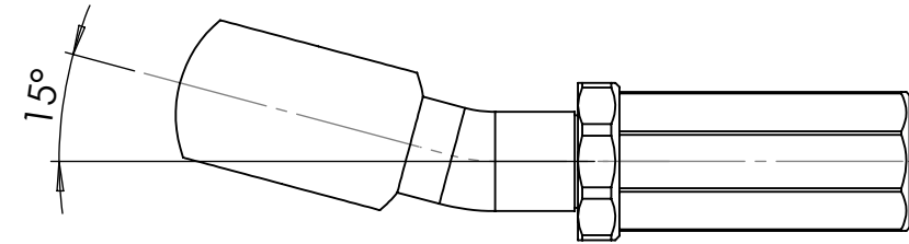
8mm banjo 15 degrees B08.15.00
