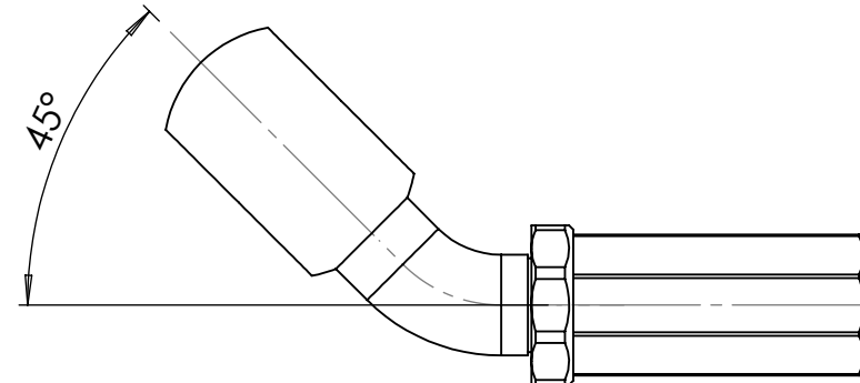
8mm banjo 45 degrees B08.45.00
