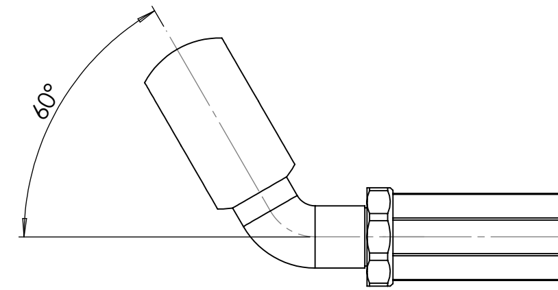
10mm banjo 60 degrees B10.60.00
