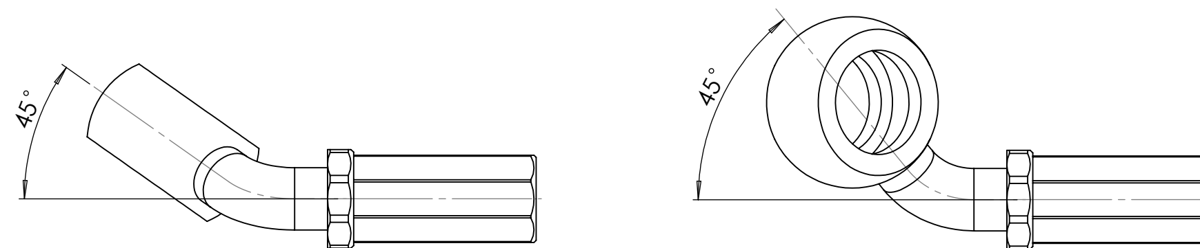
10mm banjo 45 degrees + side bend 45 degrees B10.45.45
