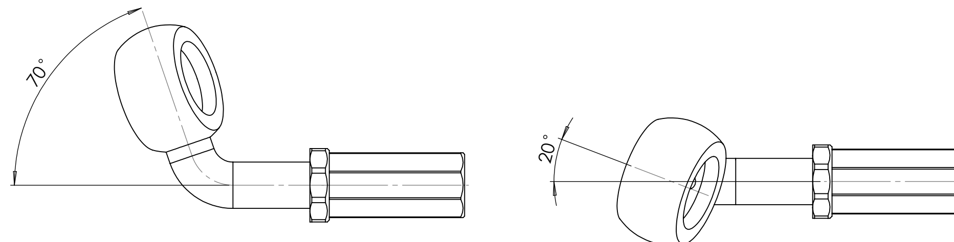
10mm banjo 70 degrees + side bend 20 degrees B10.70.20
